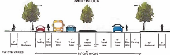
PHASE III TYPICAL SECTION MID-BLOCK
