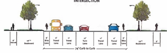
PHASE III TYPICAL SECTION INTERSECTION
