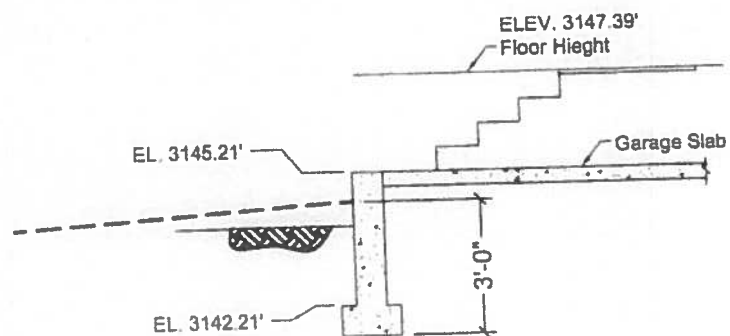
3 FOUNDATION WALL DETAIL 1/4"=1'-0"
