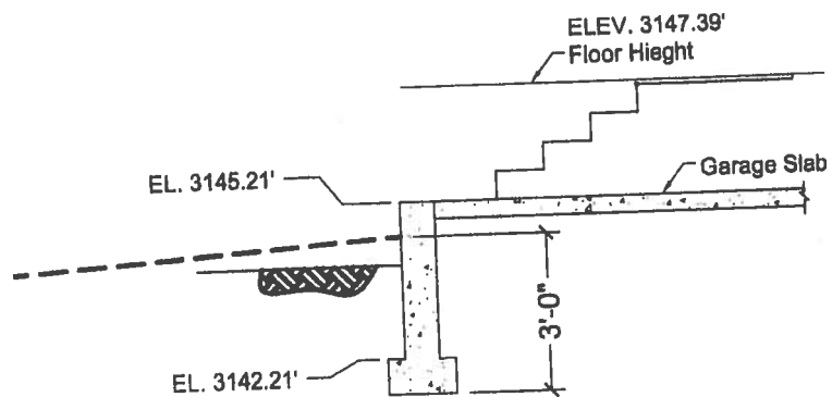
3 FOUNDATION WALL DETAIL 1/4"=1'-0"
