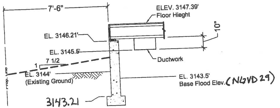
2 FOUNDATION WALL DETAIL 1/4"=1'-0"
