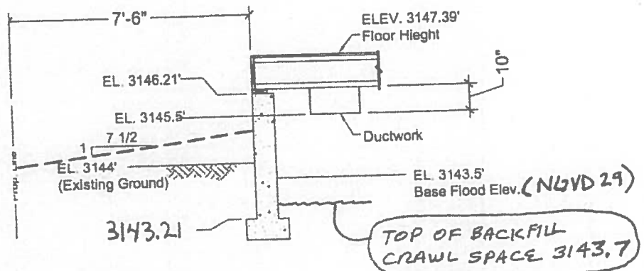
2 FOUNDATION WALL DETAIL 1/4"=1'-0"
